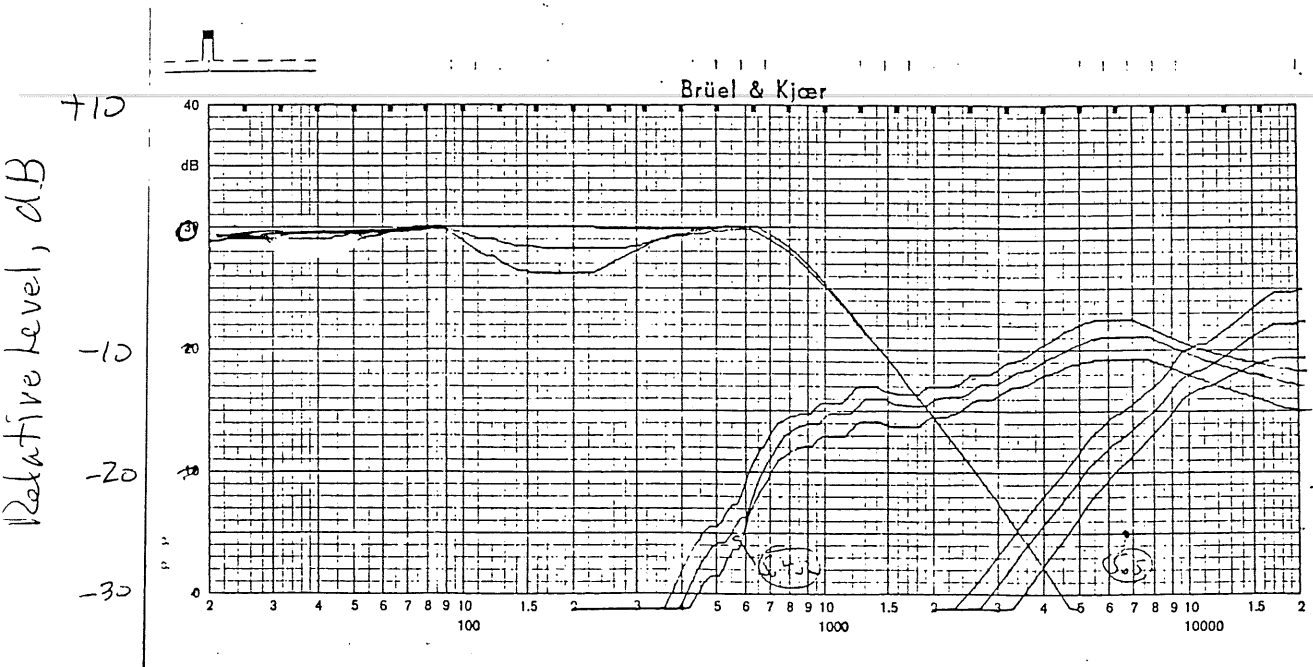
Figure 12. Voltage Drive Curves at Network Output
